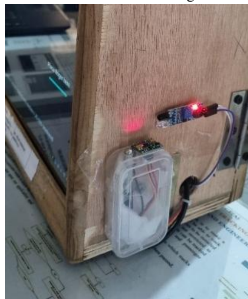
Figure.7 Thumb identification using the smart mirror
