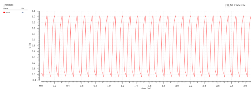
Figure 13. Simulation results with reverse bias with PMOS VCRO
