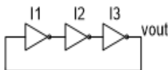
Figure 1. CMOS ring oscillator
