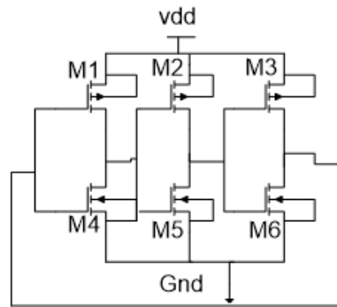
Figure 2. CMOS ring oscillator with 3 stage delay cells
