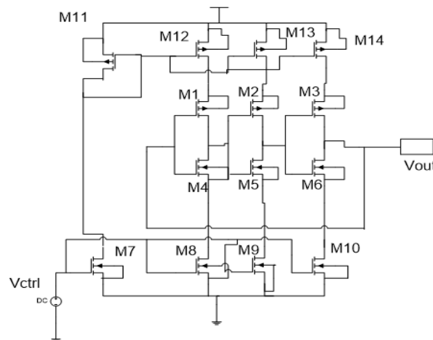
Figure 3. Current starved voltage-controlled ring oscillator (CSVCRO)
